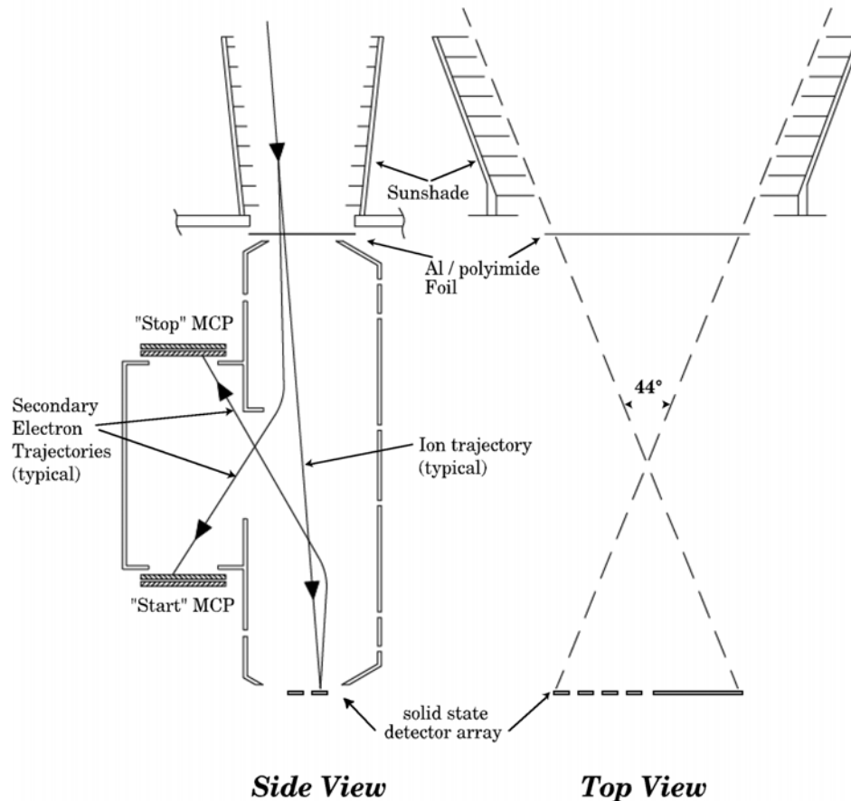
Figure 3.4.2: Cross section of the SIS Sensor
