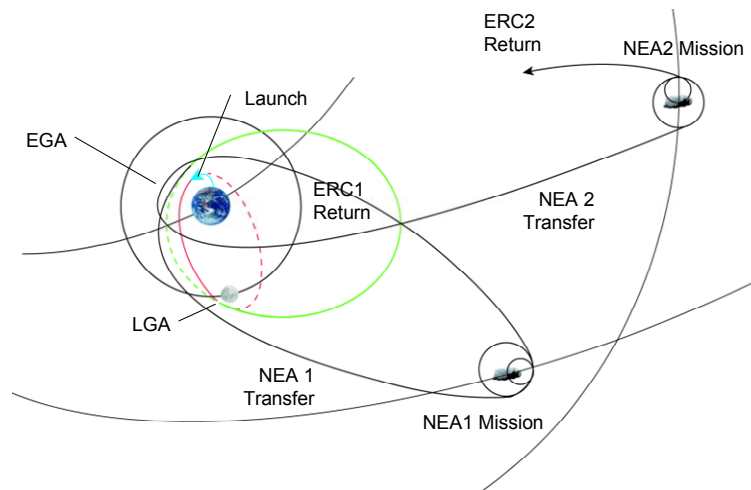
Figure 14: Alternative transfer strategy for a double asteroid mission
