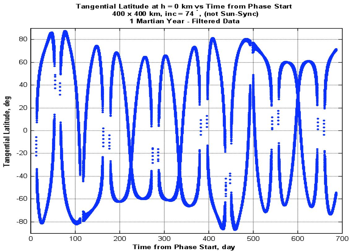
Figure 2: Solar occultation tangential latitudes versus time over a Mars year in a 400 km orbit with a 74° inclination. This shows one combination of altitude and inclination that provides latitudinal coverage each Mars season for this observational mode.
