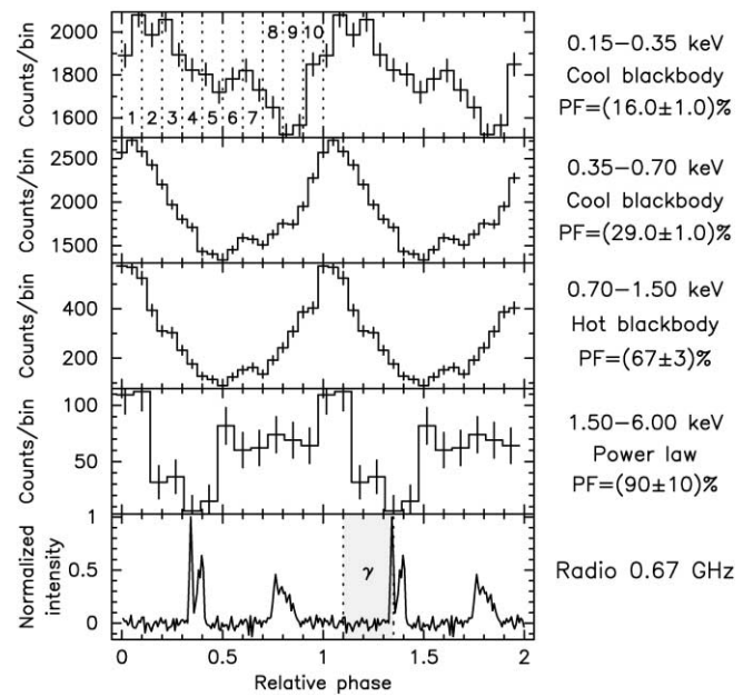
FIG. 7.—Light curves of PSR B1055–52. Note the broader profile of the X-ray pulse below 0.35 keV and the small ( \sim 0.1 ) phase shift with respect to higher energies. Note the value of the pulsed fraction, which grows with energy and is remarkably high ( \sim 70\% ) in the 0.7–1.5 keV range, where the neutron star emission is dominated by the hot blackbody component. For a more detailed study of the energy resolved pulsed fractions see Becker & Aschenbach (2002). Above 1.5 keV the low S/N hampers a detailed study of the pulse profile. We plotted the radio light curve in the bottom panel. The uncertainty on the phase alignment is of \sim 0.003 . The two radio peaks are observed to bracket the single X-ray peak. The \gamma -ray pulse (Thompson et al. 1999) occurs in the gray-shaded phase interval between the two vertical dashed lines.
