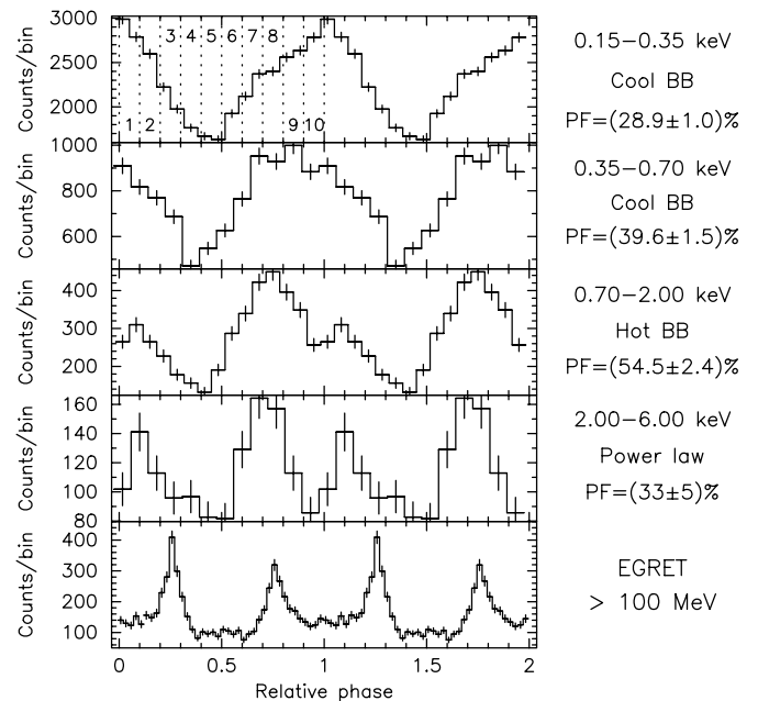
FIG. 8.—Light curves of Geminga. As discussed by Caraveo et al. (2004), the pulse shape changes as a function of energy. The single, broad peak observed at low energy (at which emission from the cool blackbody dominates) changes to two peaks at higher energies (where the power-law component dominates). The pulsed fraction is maximum in the 0.7–2 keV range, in which the hot blackbody component is more important. The bottom panels show the EGRET \gamma -ray light curve. The extrapolation of the \gamma -ray ephemeris makes the absolute phase alignment uncertain by \pm 0.15 , owing to the long time span between the EGRET and the EPIC observations. Note that the numbering of the phase intervals defined in the top panel is different from that used by Caraveo et al. (2004). Their phase 1 is phase 3 here, and similarly for the others.
