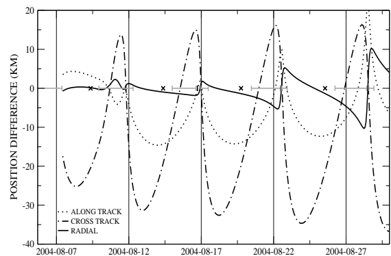
Fig. 6. Propagated orbit comparison
