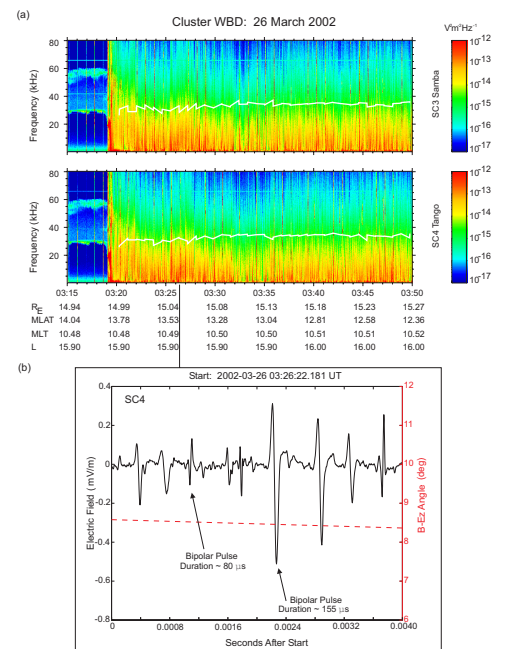
Fig.1. Example of (a) BEN observed in the magnetosheath after 03:19 UT and (b) 4 millisecond waveform showing a series of bipolar pulses which produces the broad spectrum. From Pickett et al. [17].
