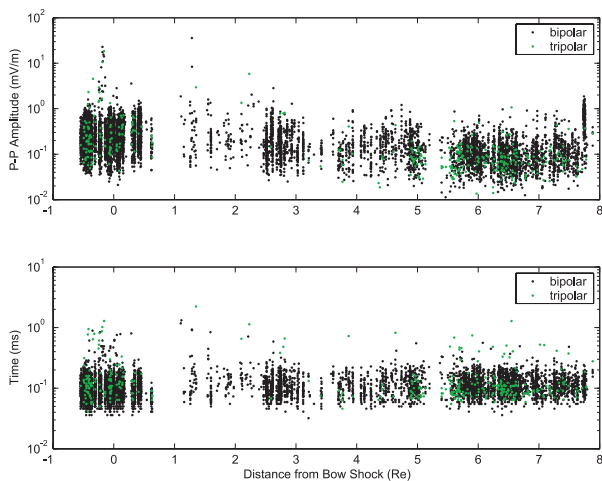
Fig. 6. Characteristics of ESWs as a function of distance from the bow shock. From Pickett et al. [17].
