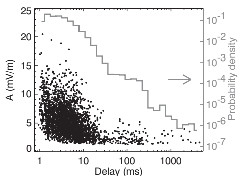
Figure 3. Scatter plot of local maxima of the amplitudes of the electric field fluctuations versus the time delays between them, as obtained from high-resolution measurements of chorus on 31 March 2001. Histogram of time delays between the local maxima is plotted by the grey line with the right-hand side vertical scale. From [Santolík et al., 2004b].
