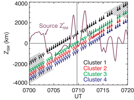
Figure 5. Z_{SM} coordinate of the four color-coded Cluster spacecraft during the geomagnetic storm on March 31, 2001, as a function of time. Sign of the parallel component of the Poynting flux is shown by downward arrows attached to the open symbols, and by upward arrows with the solid symbols, for southward and northward components, respectively. The half-filled symbols with no arrows indicate that the sign cannot be reliably determined. Horizontal grey line is at the magnetic equator, vertical grey line shows the time when center of mass of the four spacecraft crosses the equatorial plane. Shaded areas bound the regions of low values of the electromagnetic planarity. Purple line shows the calculated position where the Poynting flux changes its sign. From [Santolík et al., 2004b].
