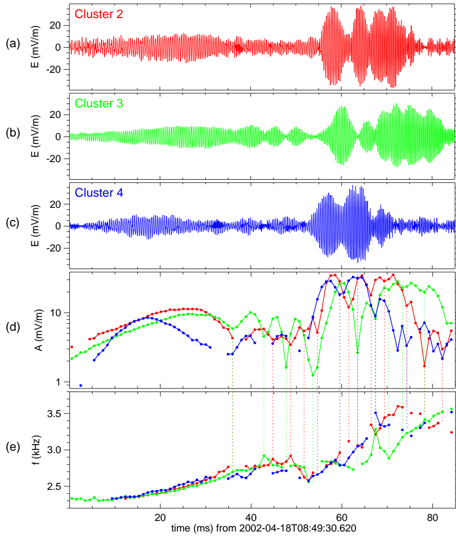
Figure 2. Waveforms and model parameters in an extended 85-ms time interval covering the second chorus element in Figure 1. (a-c) Broadband electric field waveform for Cluster 2-4, respectively; (d) Amplitude, (e) frequency. The results from the three spacecraft are color-coded. In order to demonstrate the fine structure, minima of amplitude are connected with the corresponding frequency estimates by vertical dotted lines. From [Santolík et al., 2003].
