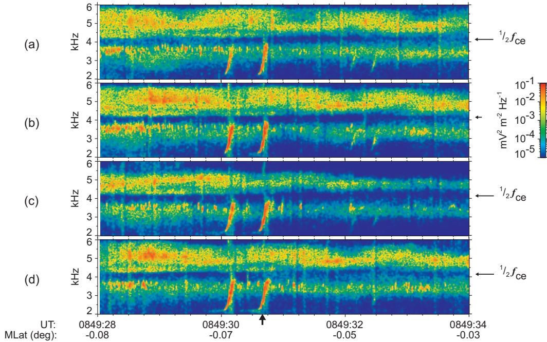
Figure 1. Detailed time-frequency power spectrograms of electric field fluctuations in the source region recorded by the WBD instruments on board all the four Cluster spacecraft on April 18, 2002 after 0849:28 UT. Panels (a-d) show data from Cluster 1-4, respectively. Horizontal arrows on the right indicate local \frac{1}{2}f_{ce} for each spacecraft. Magnetic latitude (MLat) is given on the bottom for Cluster 1. Cluster 2-4 are shifted by -0.39^\circ , -0.53^\circ , -0.25^\circ , respectively. A bold vertical arrow on the bottom points to the chorus element which is chosen for further analysis. From [Santolík et al., 2003].
