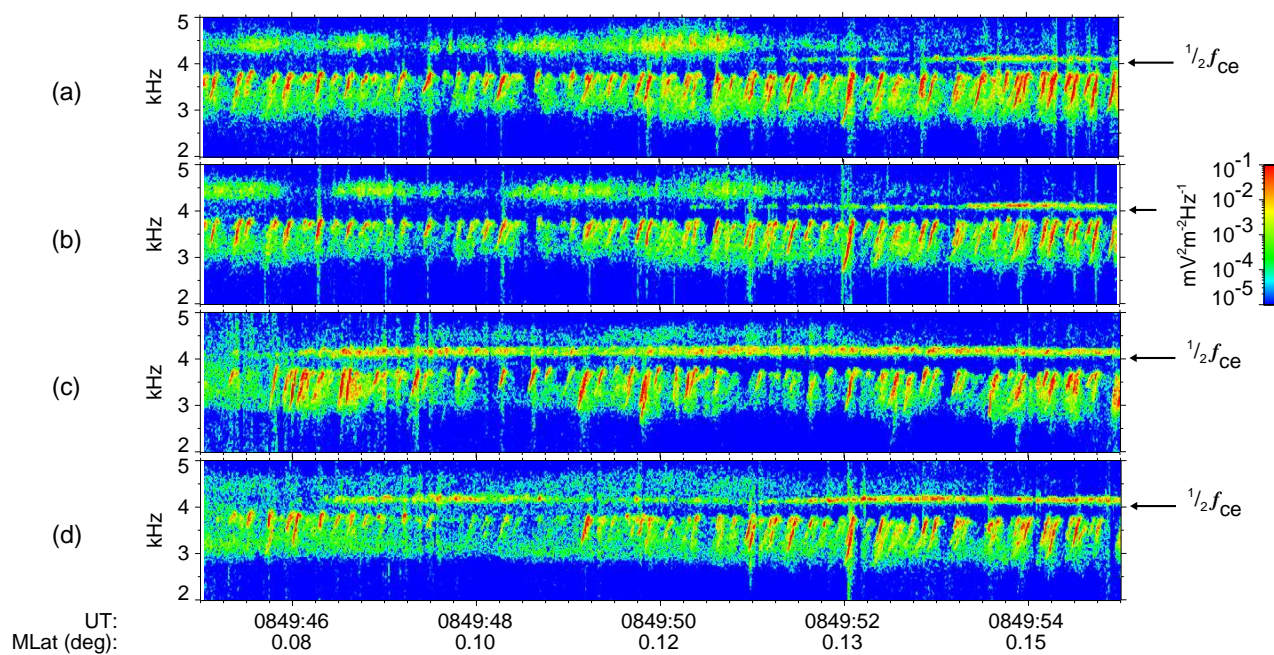
Figure 4. Detailed time-frequency power spectrograms of electric field fluctuations in the source region recorded by the WBD instruments on board the four Cluster spacecraft on April 18, 2002. Panels (a-d) show data from Cluster 1-4, respectively. Arrows indicate local \frac{1}{2}f_{ce} for each spacecraft. Magnetic dipole latitude is given on the bottom for Cluster 1. Radial distance is 4.37 R_E , and magnetic local time is 21.01 h during this interval. From [Santolík and Gurnett, 2003].
