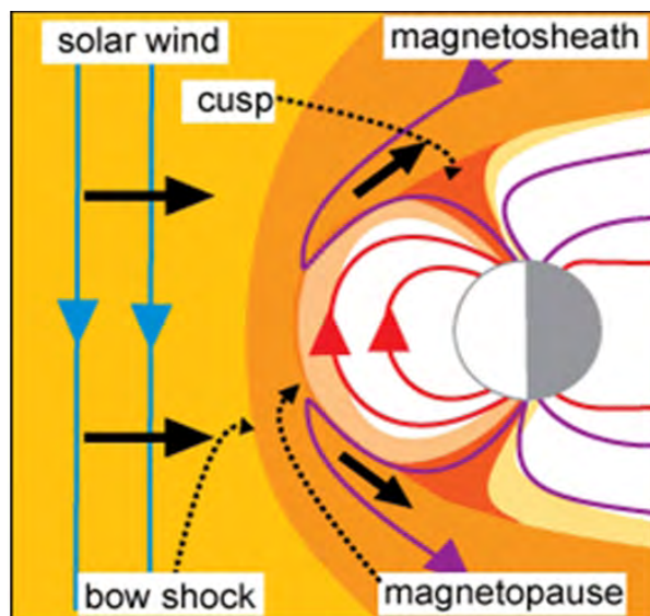
Fig. 1: The dayside magnetosphere. The magnetopause represents the outer boundary of the magnetosphere, and is compressed on the dayside. The bow shock compresses and deflects the solar wind so that it may flow around the magnetopause.
