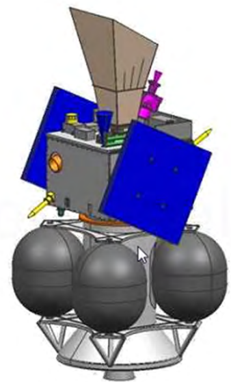
Fig. 13: Left panel – SMILE spacecraft flight configuration with its main elements labelled. Right panel – SMILE spacecraft including its propulsion module (from ESA-CAS Concurrent Design Facility)
